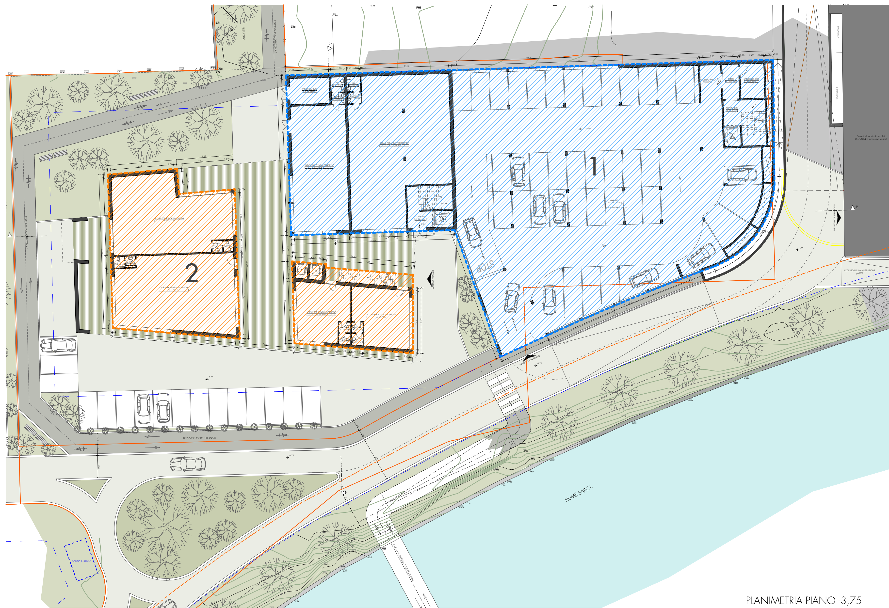
PLANIMETRIA PIANO -3,75
