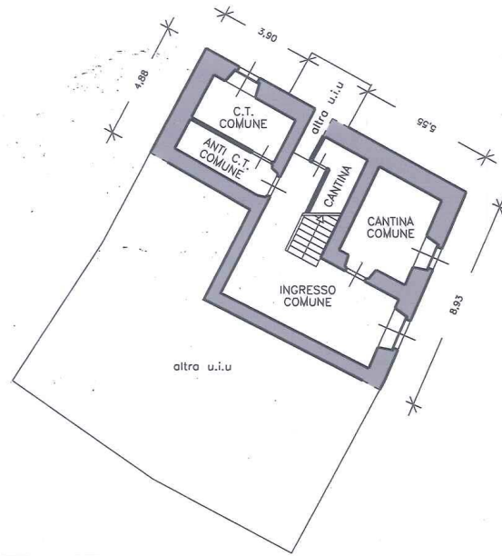
PIANO TERRA h=2,85
