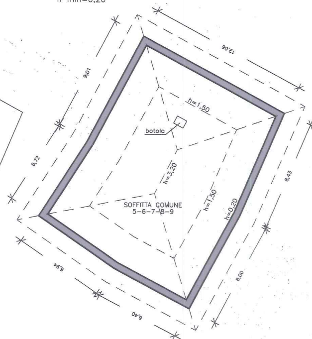
PIANO TERZO h max=3,20 h min=0,20
